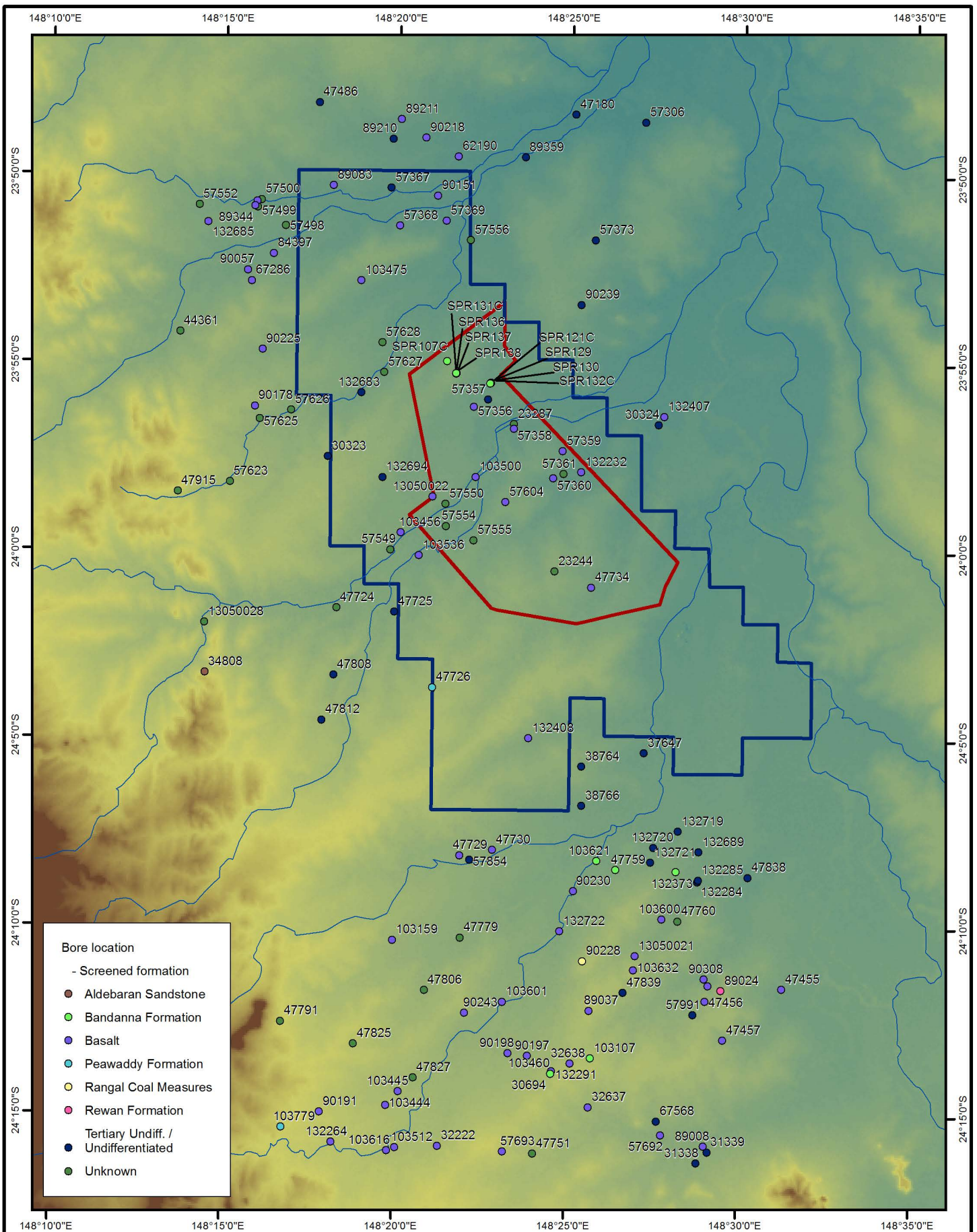
Figure 9 - 18 Bore location map
