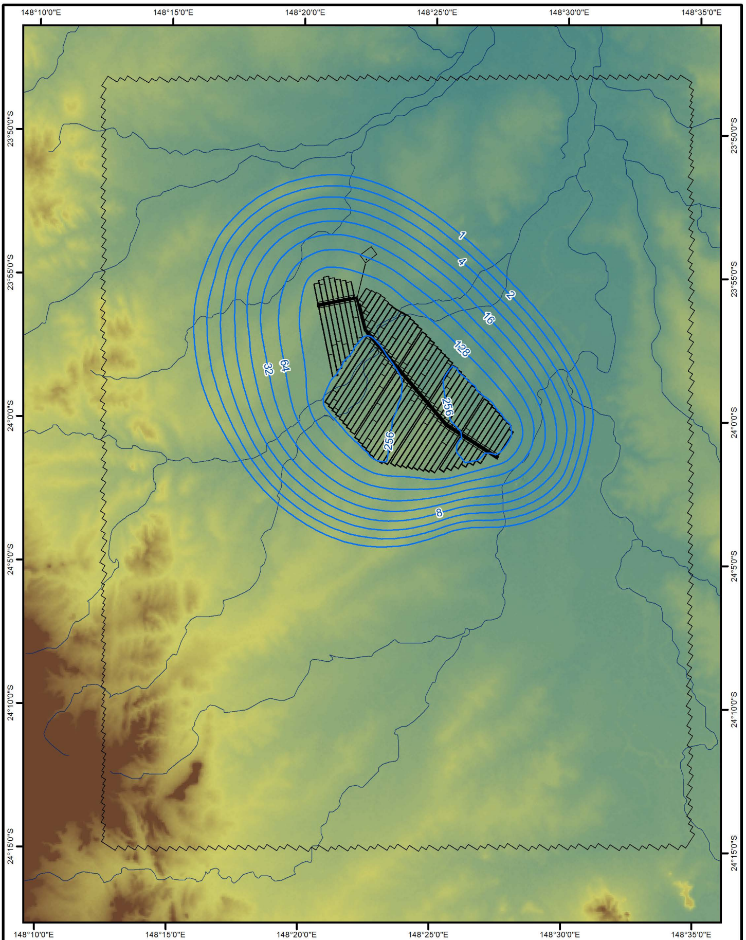
Figure 9 - 50 Drawdown in the A2 Seam after mining year 40
